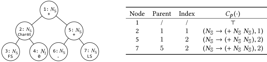
Fig. 3. An example of topdown contexts. The left figure shows the AST of program (+ (\text{CharAt } \text{FS } 0) (+ ' . ' \text{LS})) , and the right table lists the topdown contexts for some vertices of this AST.
